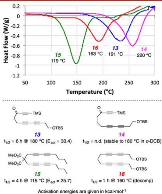
Figure 4. DSC traces for HDDA substrates lacking fully conjugated tethers: Ynones 13 and 14 and tetraynes 15 and 16.
